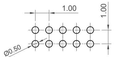
Recommended PCB Layout General TOL: ±0.05
